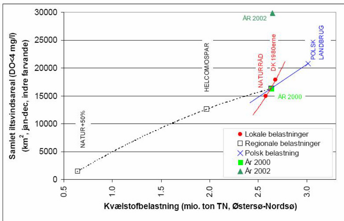
Figure 14.2: Annual extent of oxygen depletion ( < 4 \text{ mg O}_2/\text{l}</math>) in the Danish coastal waters as a function of the nitrogen load (water and air-borne).
