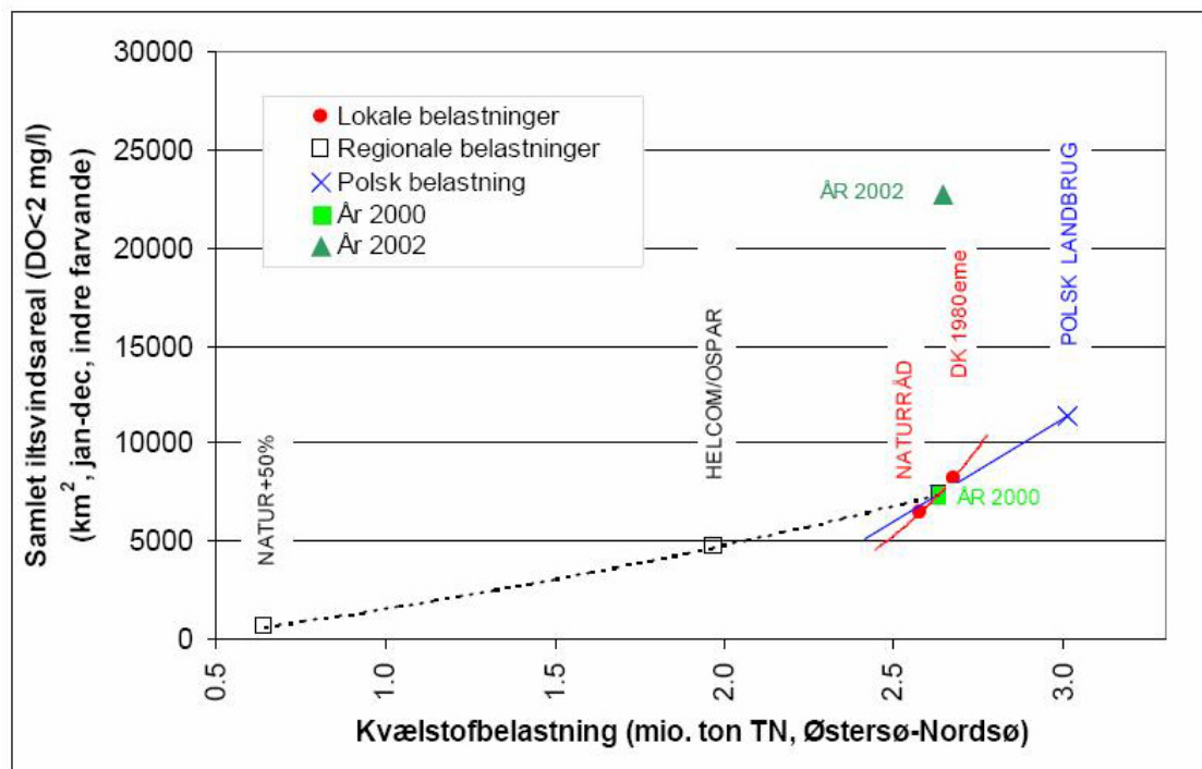
Figure 14.3: Annual extent of oxygen depletion ( < 2 \text{ mg O}_2/\text{l}</math>) in the Danish coastal waters as a function of the annual nitrogen load (water and air-borne).
