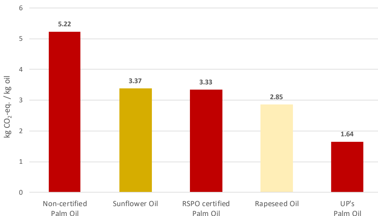
Figure 5.1: GHG emission of UP's palm oil calculate in this report, average palm oil (Schmidt and De Rosa 2019), sunflower oil and rapeseed oil (Schmidt and De Rosa 2019; Schmidt 2015) with iLUC and nature conservation. The chart shows the results for RSPO certified and non-certified RBD palm oil in 2016 and for UP's NBD palm oil in 2019. The results for RSPO certified and non-certified palm oil are slightly different (-2%) than in Schmidt and De Rosa (2019) due to updated values of capital goods and services and dinitrogen oxides emissions.
