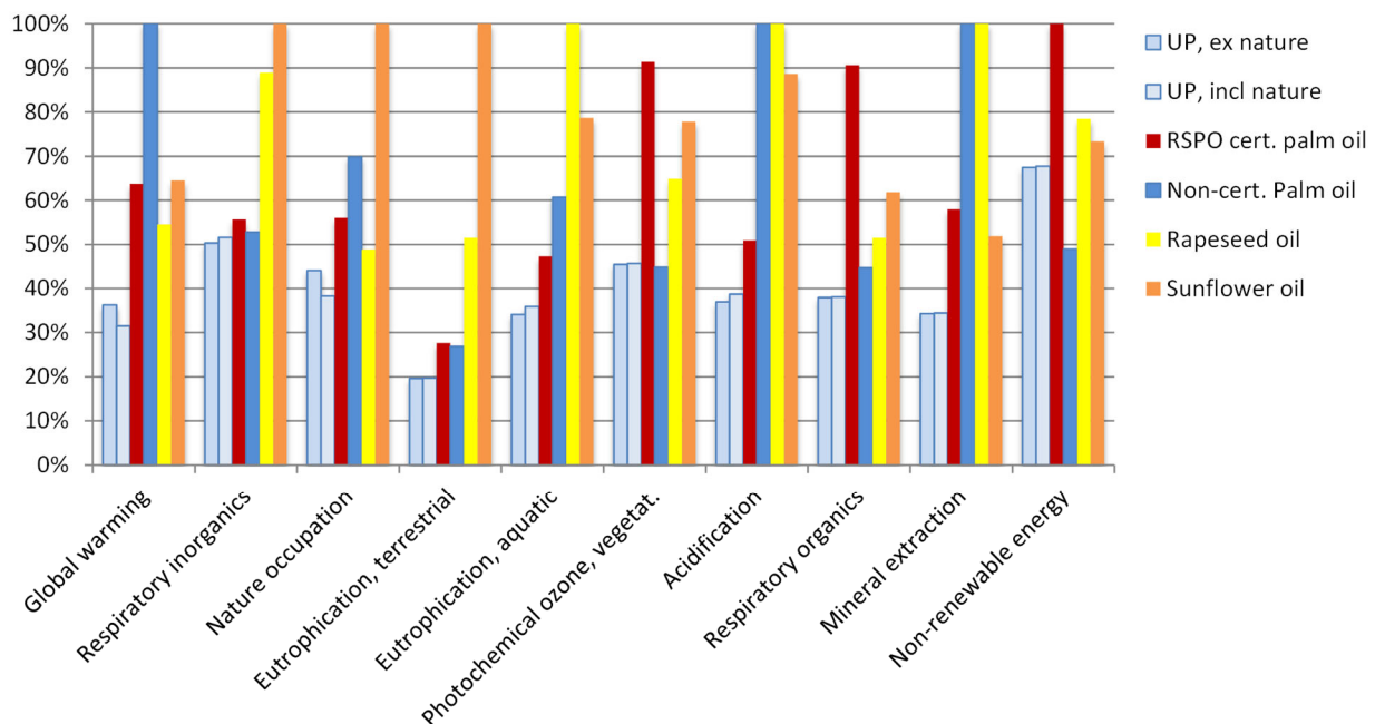
Figure 4.5: Comparison of LCIA results (including only iLUC and both iLUC and nature conservation) for 1 kg NBD palm oil at United Plantations Berhad in 2019 with industry averages for 2016 for palm oil (Malaysia and Indonesia), rapeseed oil (Europe) and sunflower oil (Ukraine).
