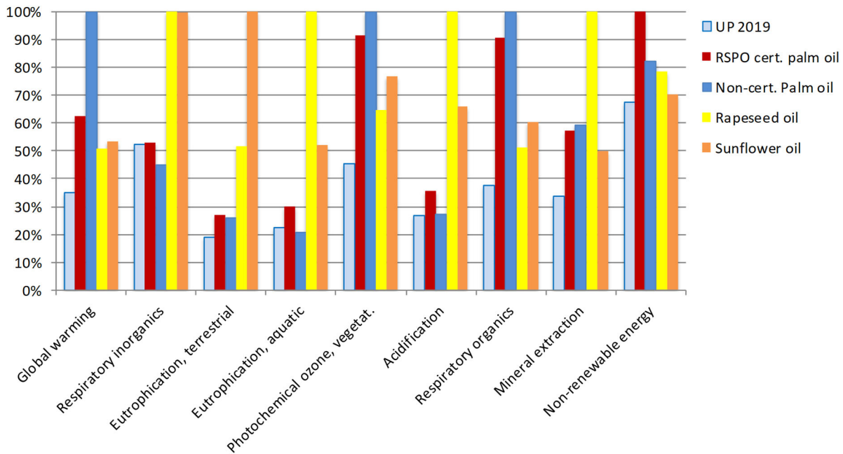
Figure 4.4: Comparison of LCIA results (excluding iLUC) for 1 kg NBD palm oil at United Plantations Berhad in 2019 with industry averages for 2016 for palm oil (Malaysia and Indonesia), rapeseed oil (Europe) and sunflower oil (Ukraine).
