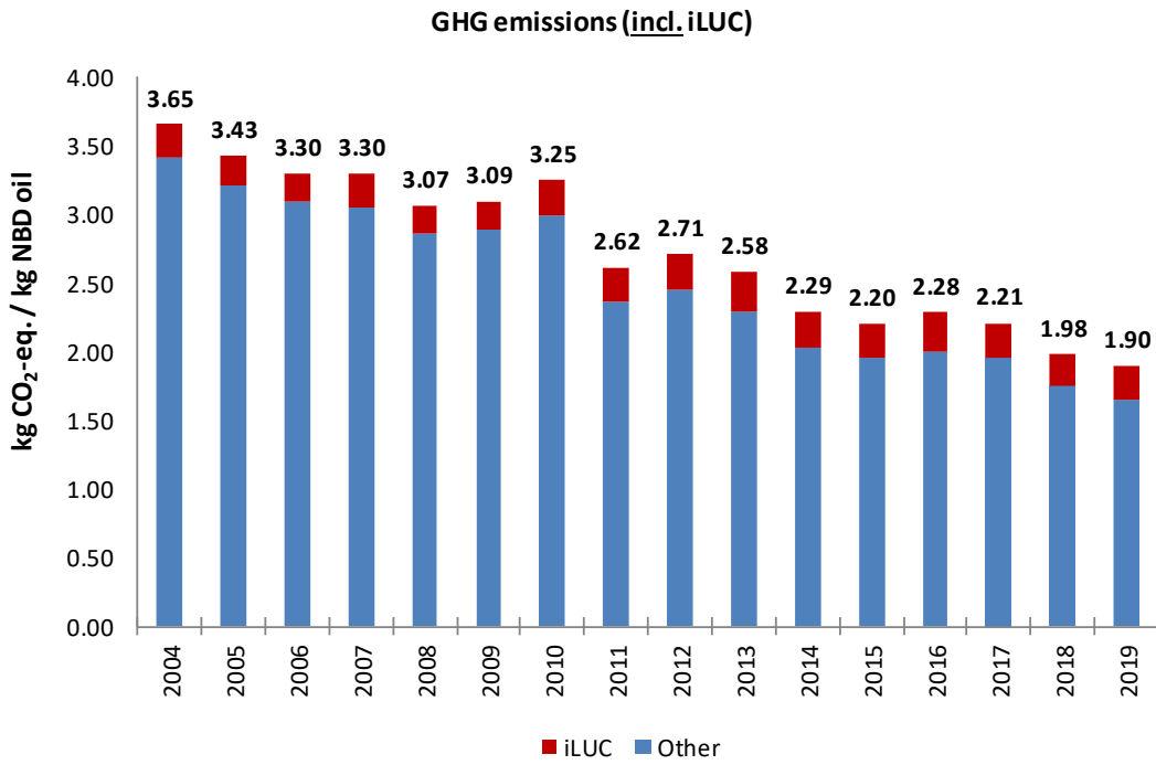
Figure 4.2: Time-series for NBD palm oil at United Plantations Berhad (with iLUC and without nature conservation) for 2004-2019.
