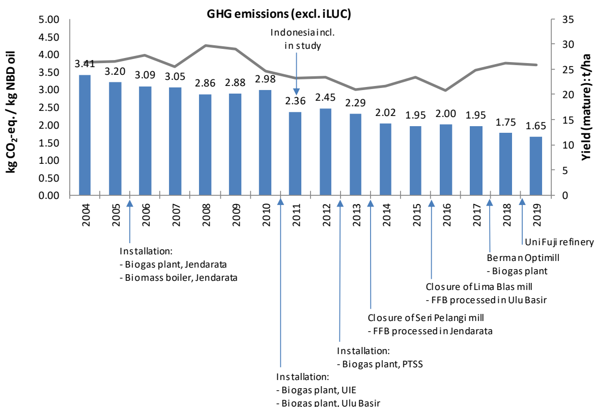
Figure 4.1: Time-series for NBD palm oil at United Plantations Berhad (without iLUC and without nature conservation) for 2004-2019.
