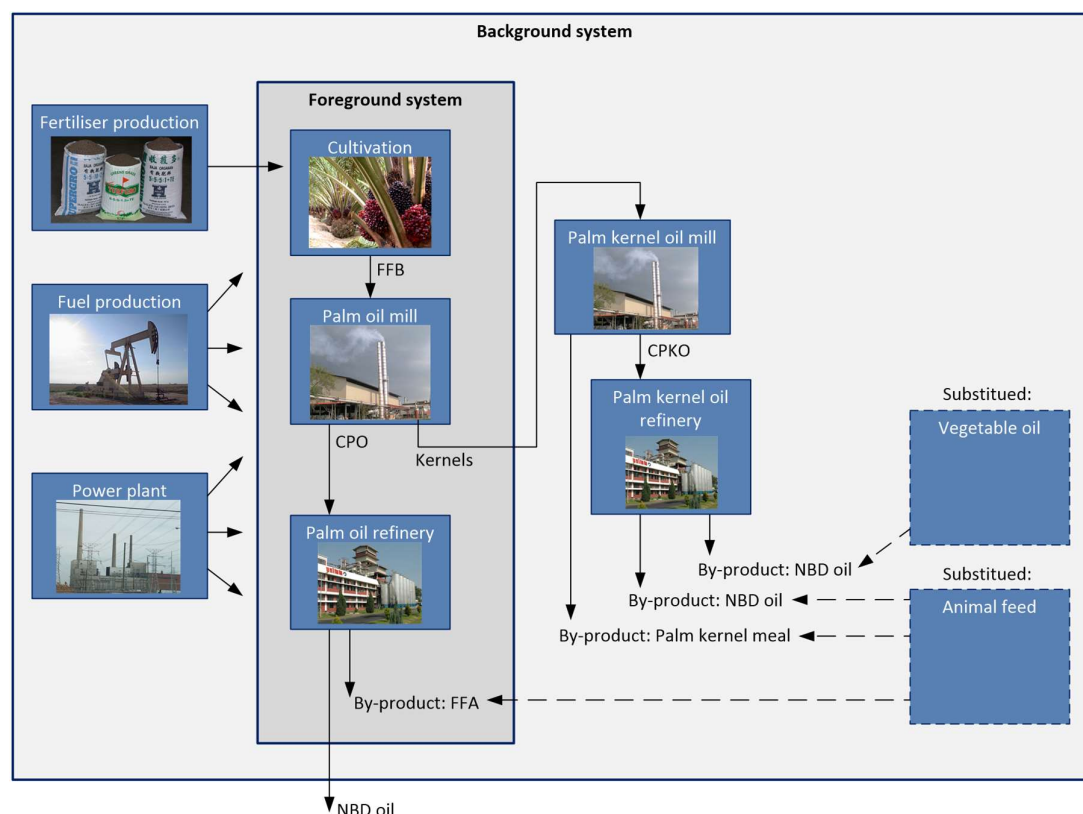
Figure 2.1: The main stages of the product system for palm oil production. Dotted lines and boxes represent negative flows and substituted activities respectively. The FFA (free fatty acid) is also sometimes referred to as palm acid oil (PAO). Pictures: UP picture library and Wikipedia.
