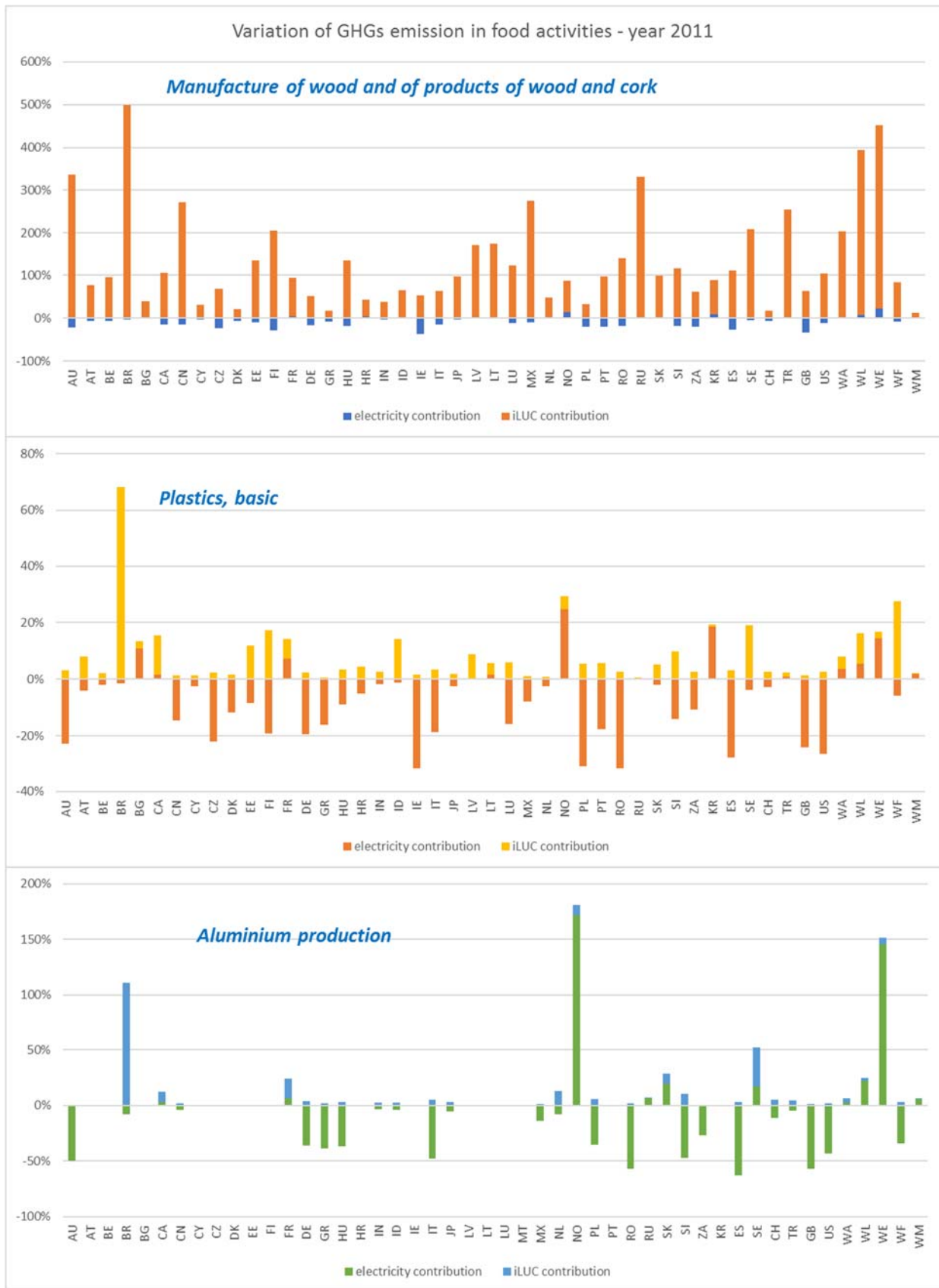
Figure 11 - Effect on GHGs emissions in three manufactural activities when applying the electricity and iLUC models to EXIOBASE v.3.3.11. The charts show the variation in percentage per dry-matter unit.
