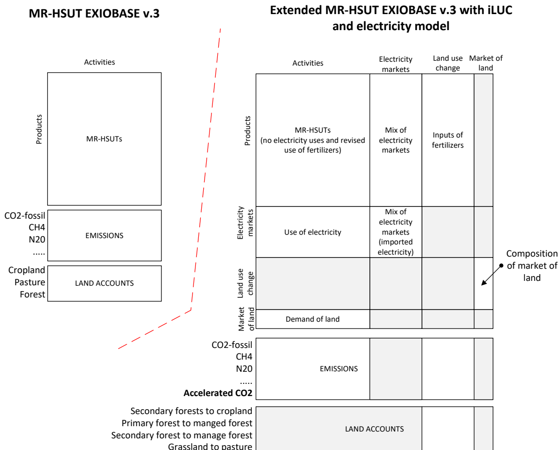
Figure 0 – Extended version of EXIOBASE v.3 with iLUC and electricity models. On the left side it is shown the structure of original MR-HSUTs EXIOBASE v.3 while on right the changed occurred when applied the electricity and iLUC models. The grey area indicates that no data are there included in.
