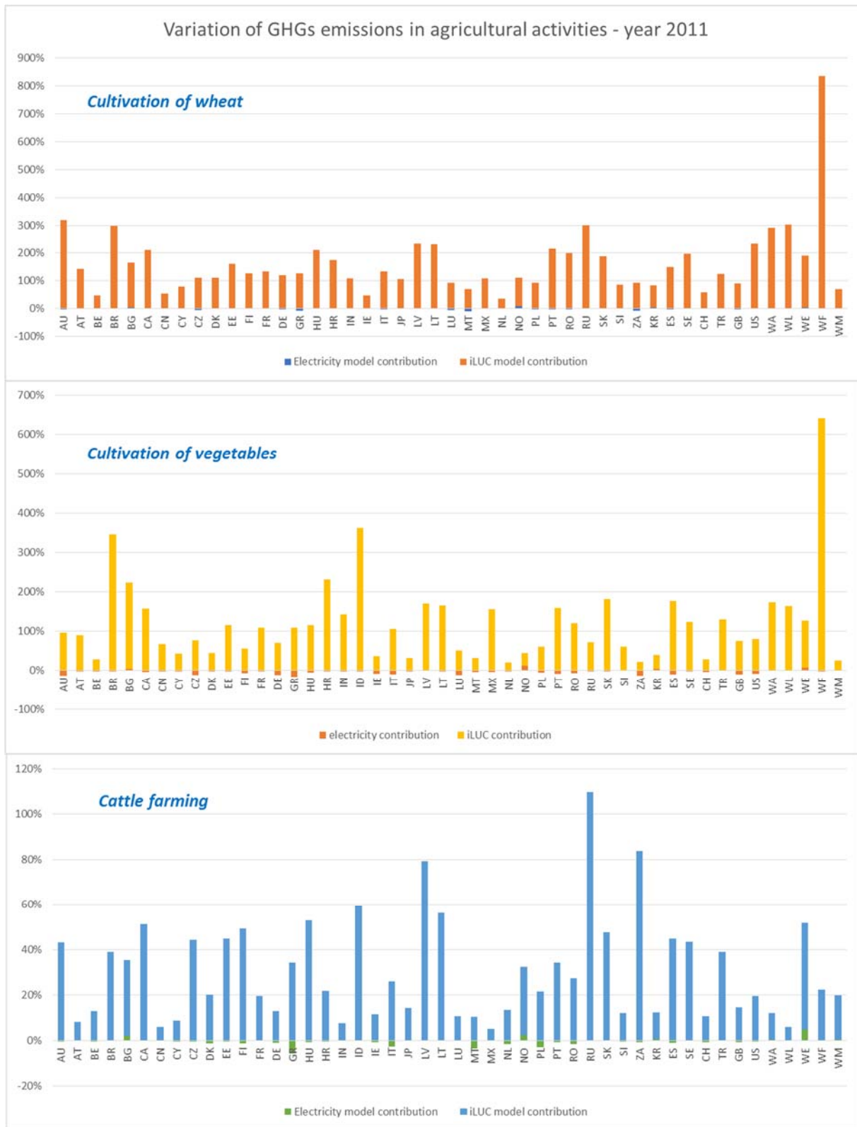
Figure 9 – Effect on GHGs emissions in three agricultural activities when applying the electricity and iLUC models to EXIOBASE v.3.3.11. The charts show the variation in percentage per dry-matter unit.
