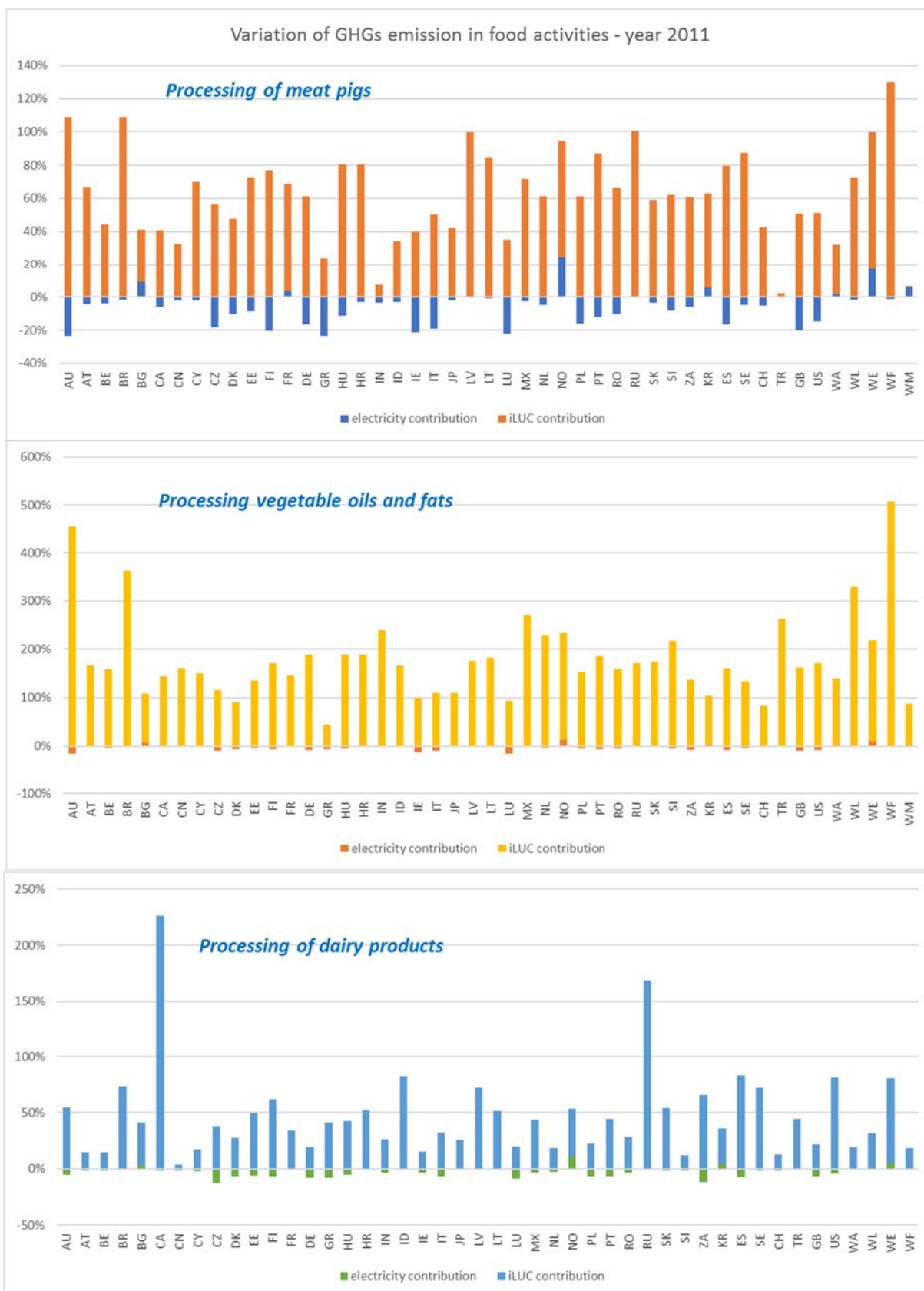
Figure 10 - Effect on GHGs emissions in three food activities when applying the electricity and iLUC models to EXIOBASE v.3.3.11. The charts show the variation in percentage per dry-matter unit.
