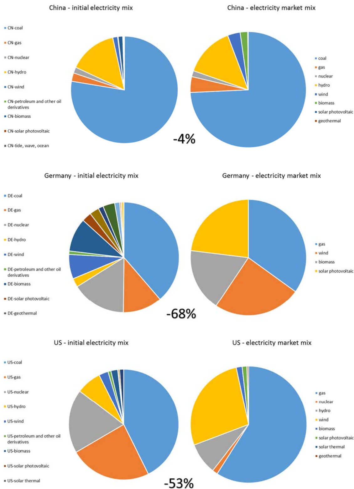
Figure 6 – Comparison of electricity mixes in the standard EXIOBASE v.3.3.11 (left pie) and the extended version (right pie) for three main economies in 2011. The percentages between the two national chart shows the variation of GHGs emissions when implementing the electricity model.
