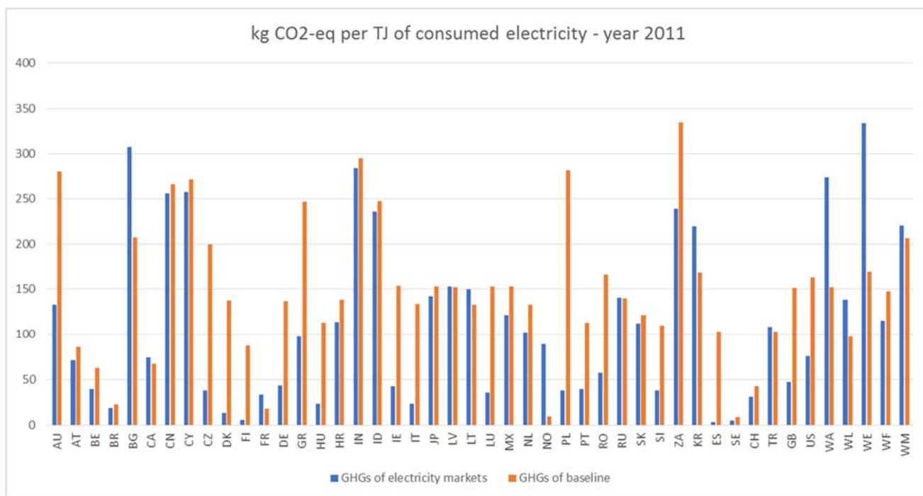
Figure 8 – Comparison of greenhouses gas emission per unit of consumed electricity in the EXIOBASE regions when applying the electricity model. Left bar shows the impact of the electricity markets, the right bar the impact in the baseline.
