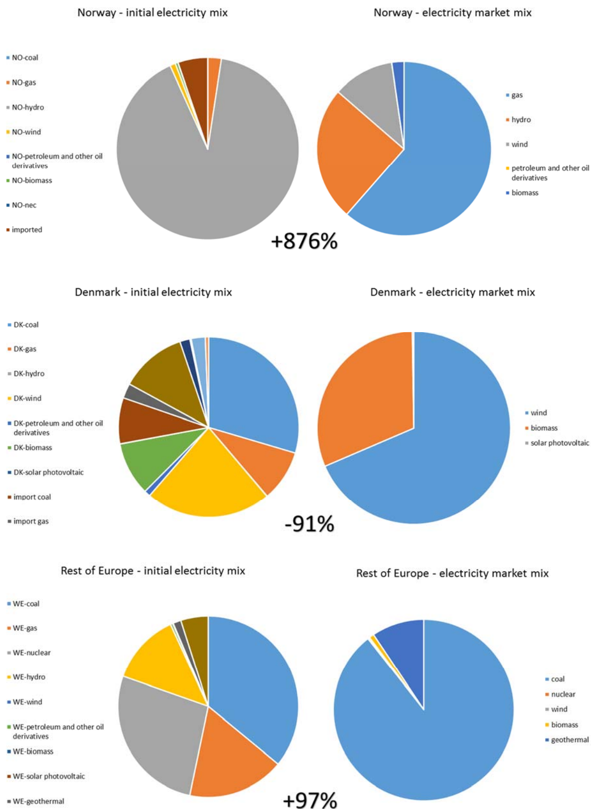
Figure 7 - Comparison of electricity mixes in the standard EXIOBASE v.3.3.11 (left pie) and the extended version (right pie) for three areas with the highest variation of GHGs emissions in 2011. The percentage between the two charts indicates the variation due to introduction of electricity markets.
